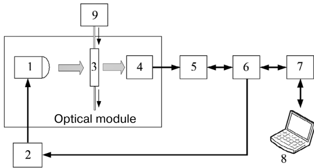
Fig. 2. Block diagram of the dual-wavelength sensor.
